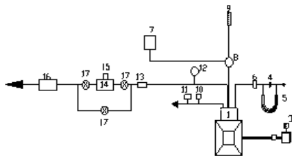
Fig.1. Experimental Setup for Pure Diesel Operation
